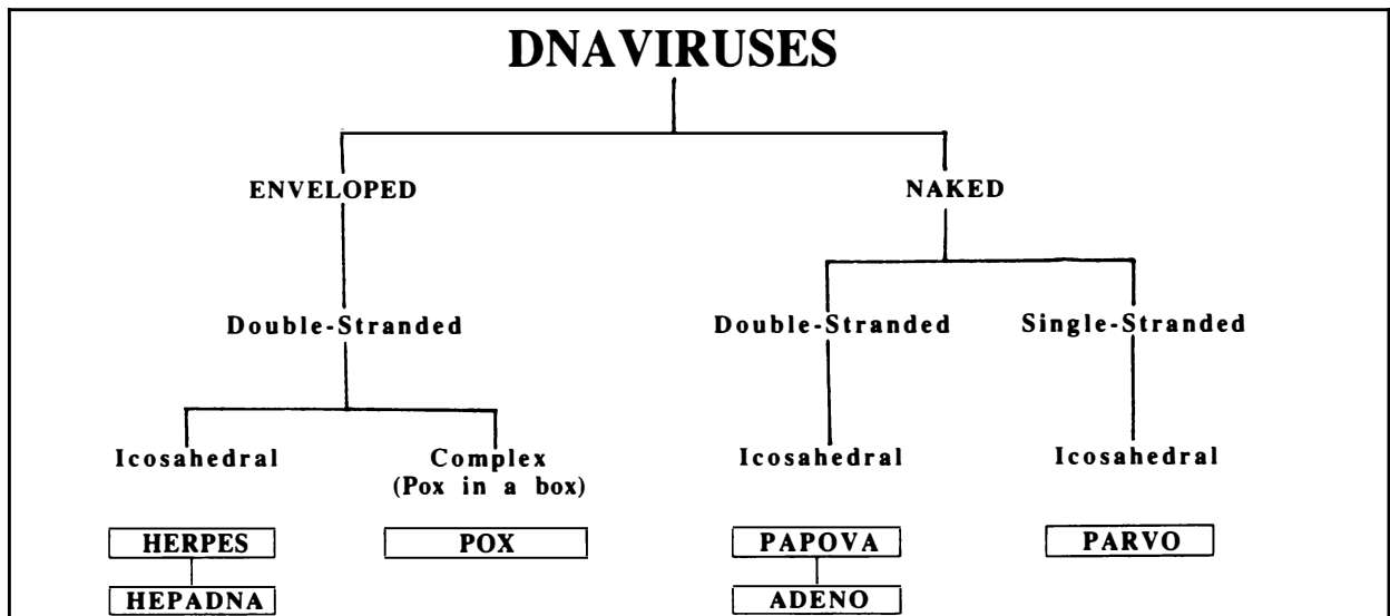
Figure 23-13 DNA VIRUSES
