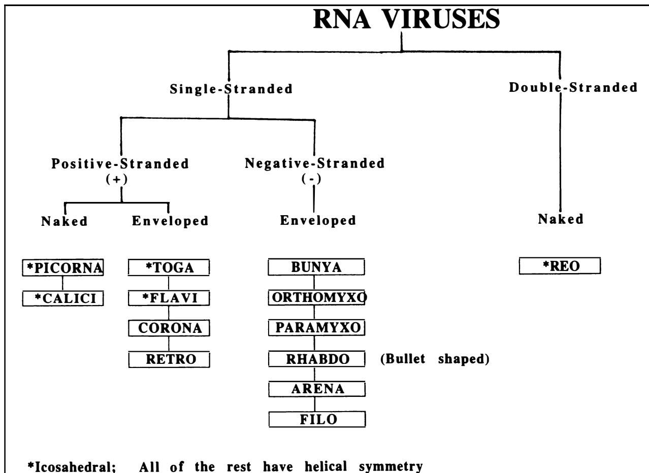
Figure 23-14 RNA VIRUSES
