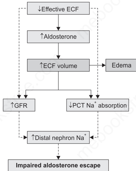
Fig. 17.13: Impaired aldosterone escape mechanisms in hyper-volemic states. Broke line indicates inhibitory pathway
