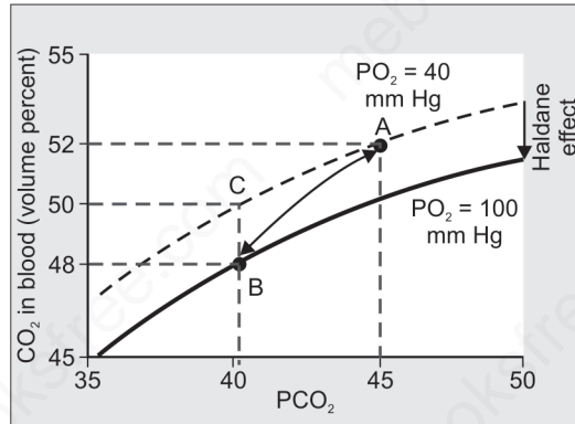
Fig. 10.6: Portions of the carbon dioxide dissociation curve when the PO 2 is 100 mm Hg or 40 mm Hg. The arrow represents the Haldane effect on the transport of carbon dioxide, as discussed in the text
