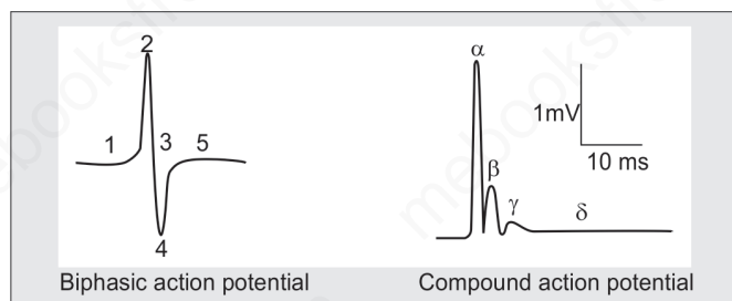
Fig. 3.10: Biphasic and compound action potential
